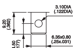
Sold. lug/Quick-connect
