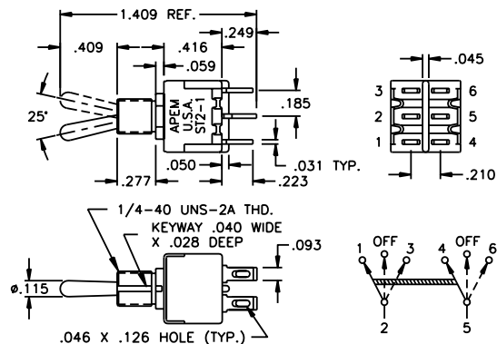
DOUBLE POLE
