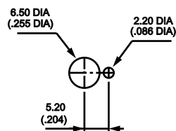
Panel Cut-out
