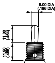
12 Short lever
