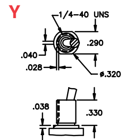
Y LONG THREADED
