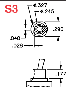
S3 NON THREADED
