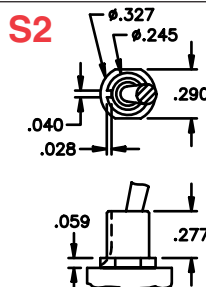
S2 NON THREADED
