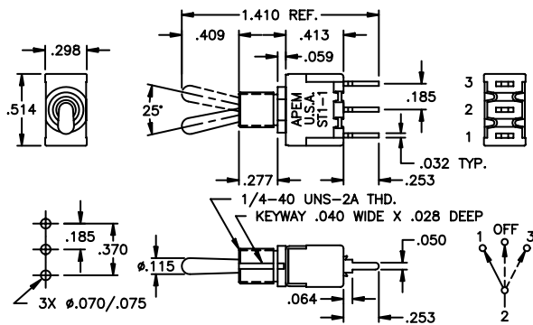
SINGLE POLE
