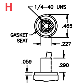
H SPLASHPROOF
