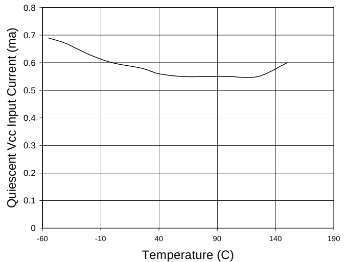
Fig. 22 Quiescent Supply Current vs. Temperature V CC = 18V, Vin = 5V@1kHz, CL = 1000pF
