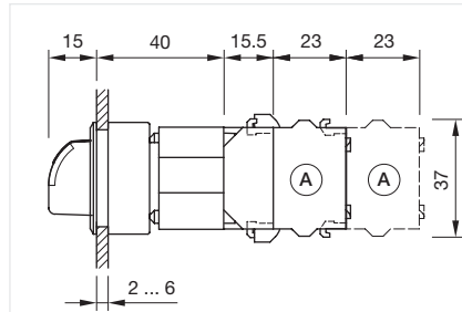
Dimensions [mm] A = Screw terminal X = Screw terminal
