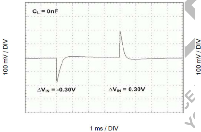
Figure 10. Line Transient Response
