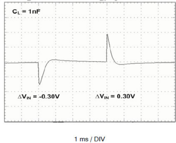
Figure 11. Line Transient Response with Cap. Load
