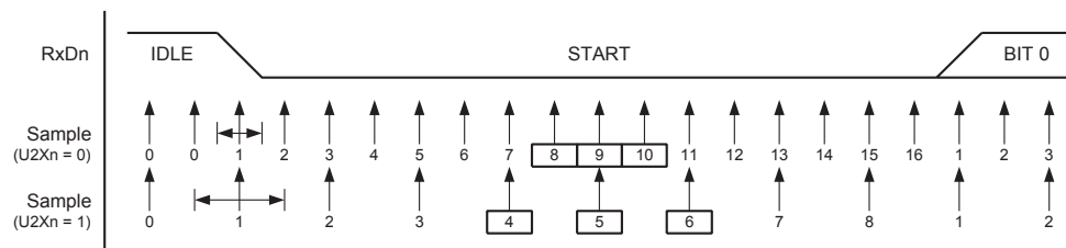
Figure 84. Start Bit Sampling
