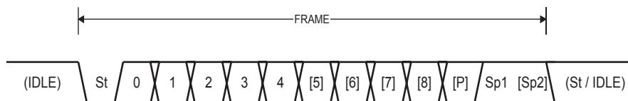
Figure 83. Frame Formats
