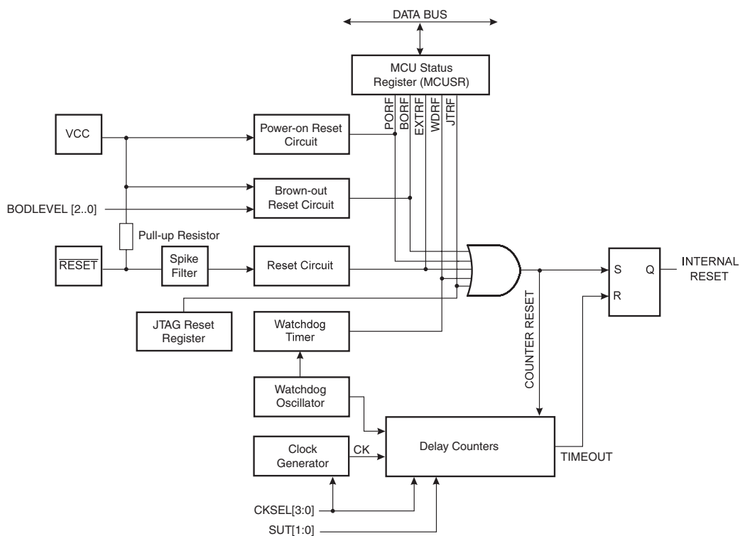
Figure 22. Reset Logic
