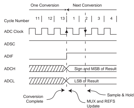
Figure 130. ADC Timing Diagram, Free Running Conversion
