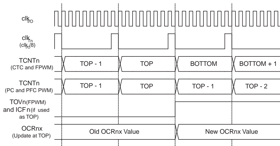
Figure 59. Timer/Counter Timing Diagram, with Prescaler ( f_{clk\_I/O}/8 )
