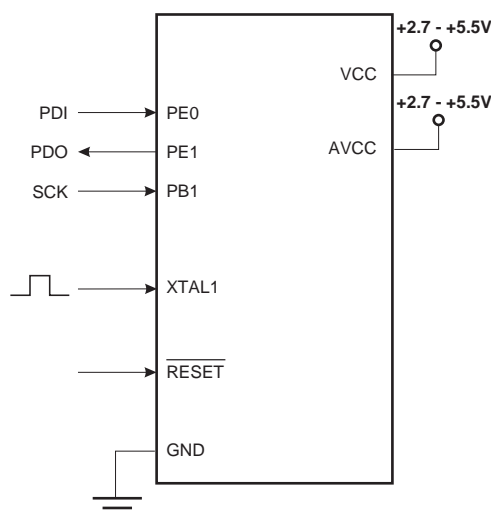
Figure 159. Serial Programming and Verify (1)
