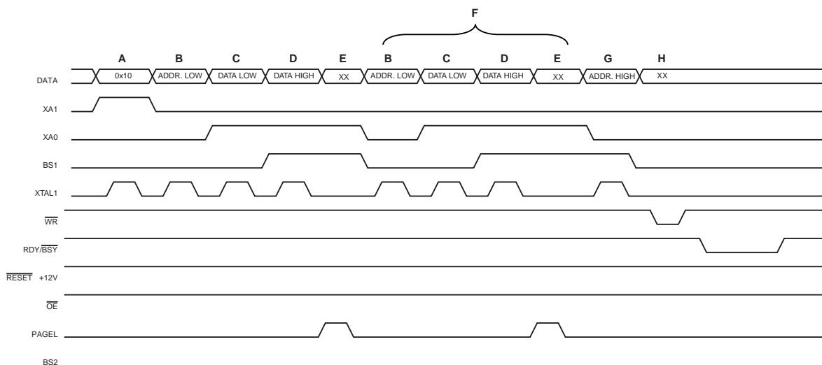
Figure 155. Programming the Flash Waveforms (1)
