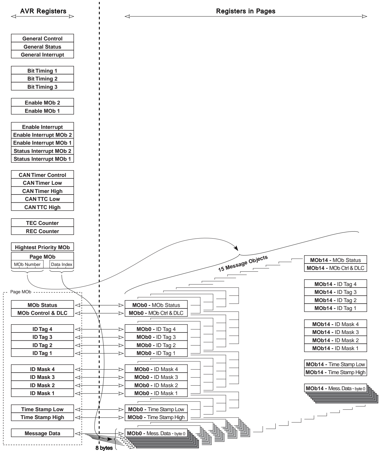
Figure 122. Registers Organization
