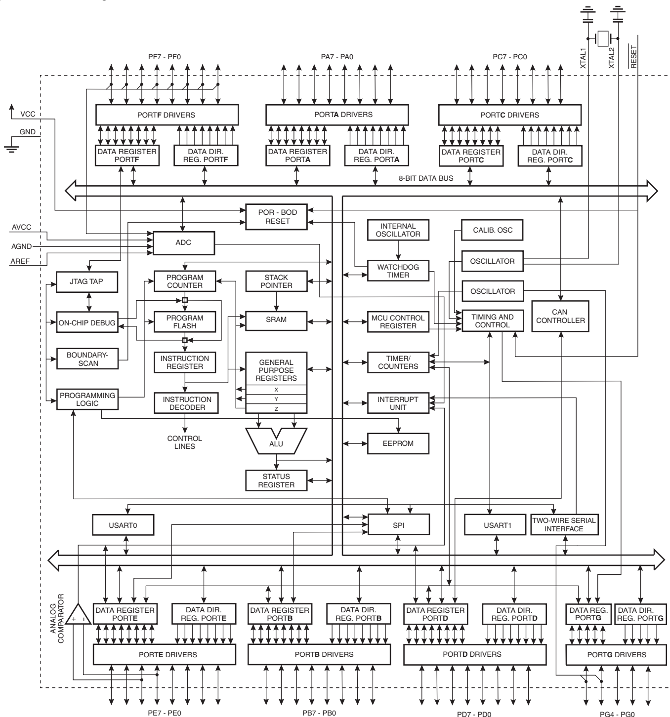
Figure 1. Block Diagram
