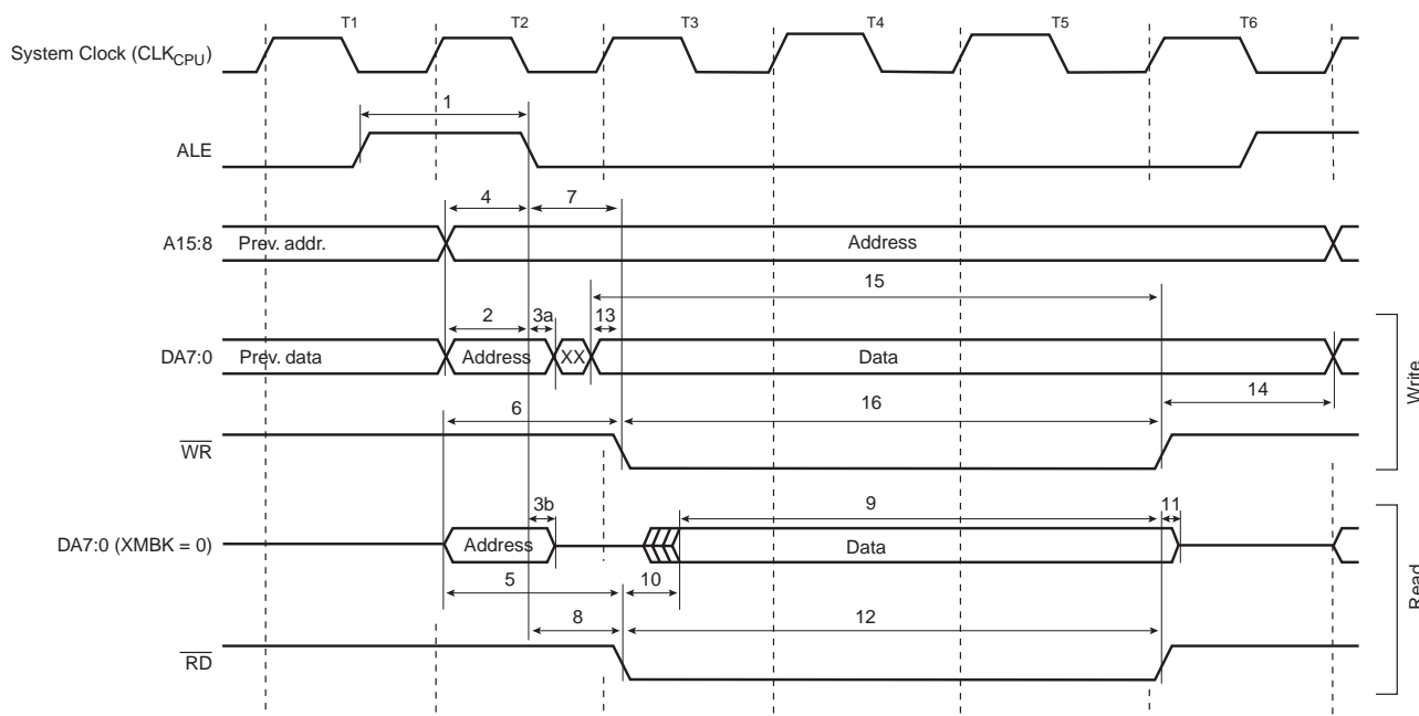
Figure 172. External Memory Timing (SRWn1 = 1, SRWn0 = 0)
