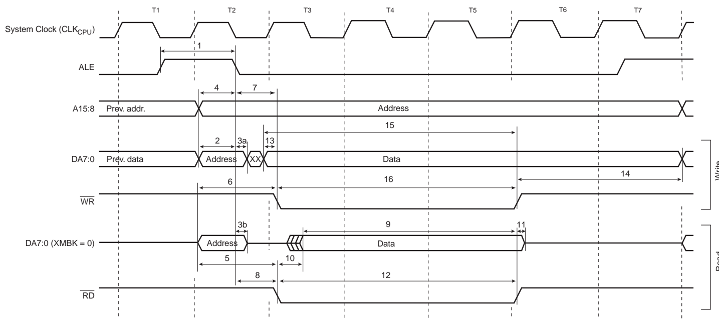
Figure 173. External Memory Timing (SRWn1 = 1, SRWn0 = 1) (1)
