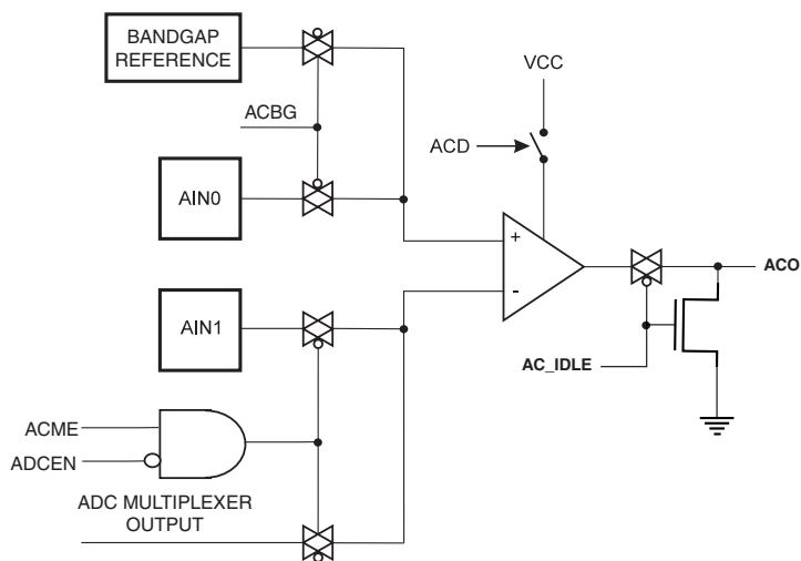
Figure 147. Analog Comparator
