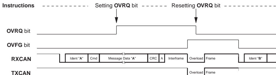
Figure 116. Overload Frame
