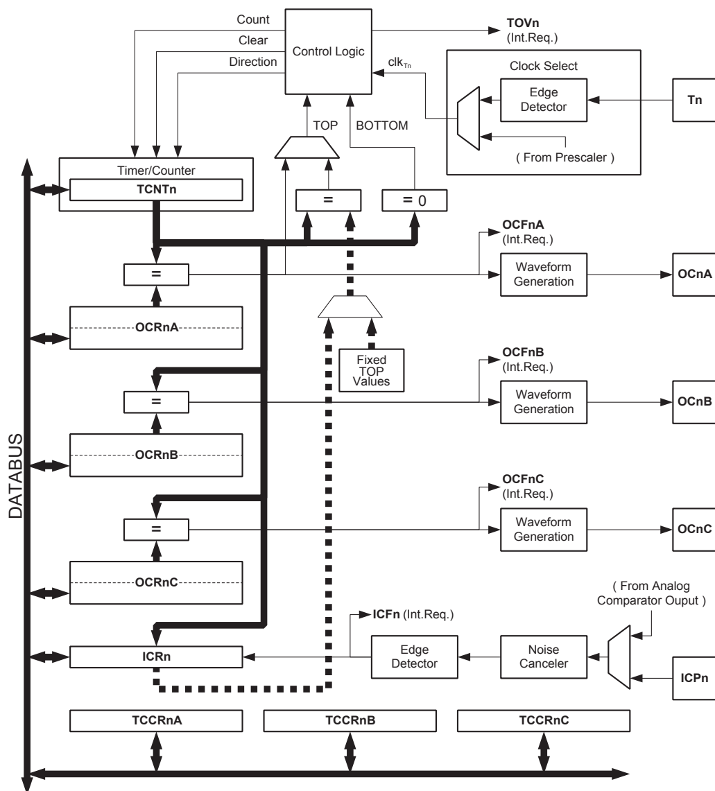
Figure 47. 16-bit Timer/Counter Block Diagram (1)
