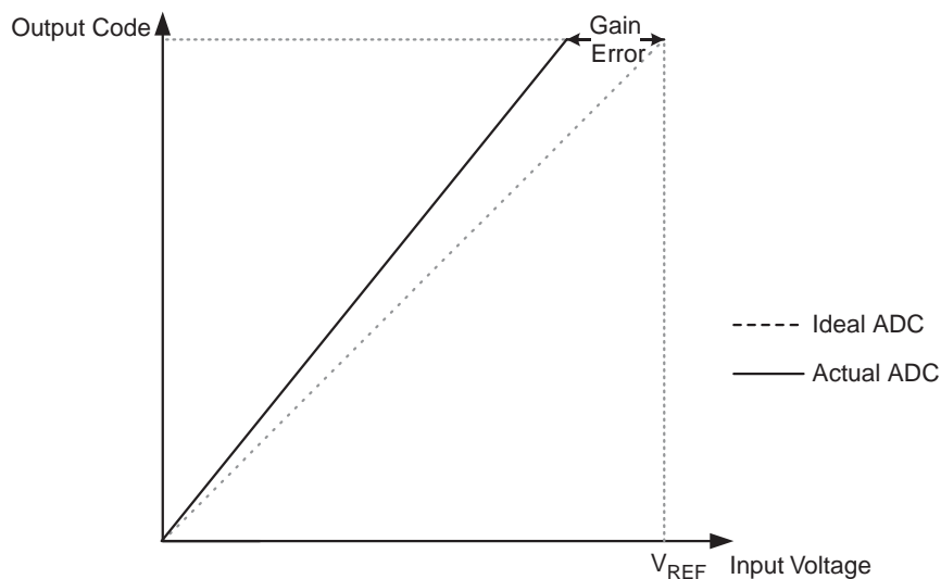
Figure 134. Gain Error
