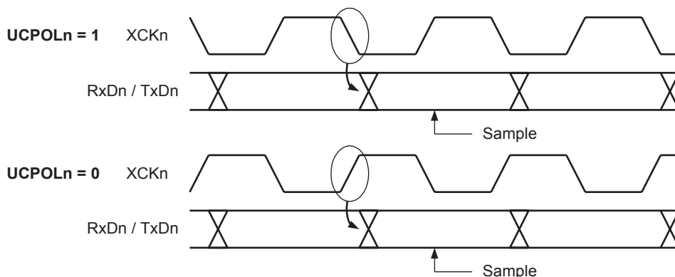
Figure 82. Synchronous Mode XCKn Timing.
