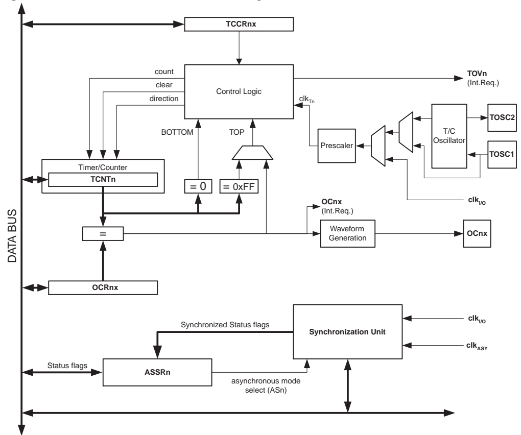
Figure 60. 8-bit Timer/Counter2 Block Diagram
