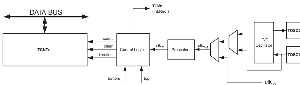
Figure 61. Counter Unit Block Diagram
