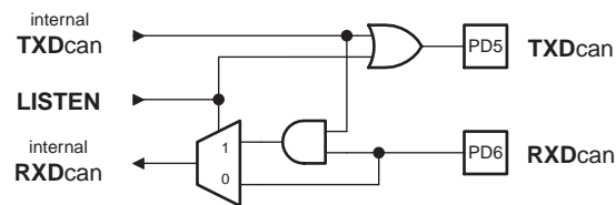
Figure 113. Listening Mode
