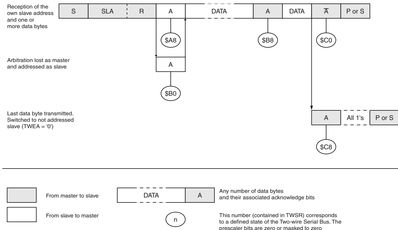
Figure 104. Formats and States in the Slave Transmitter Mode
