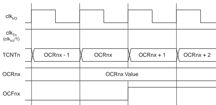
Figure 56. Timer/Counter Timing Diagram, Setting of OCFnx, no Prescaling
