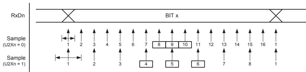
Figure 85. Sampling of Data and Parity Bit
