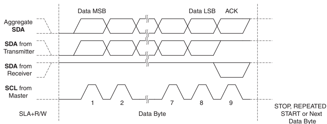
Figure 91. Data Packet Format
