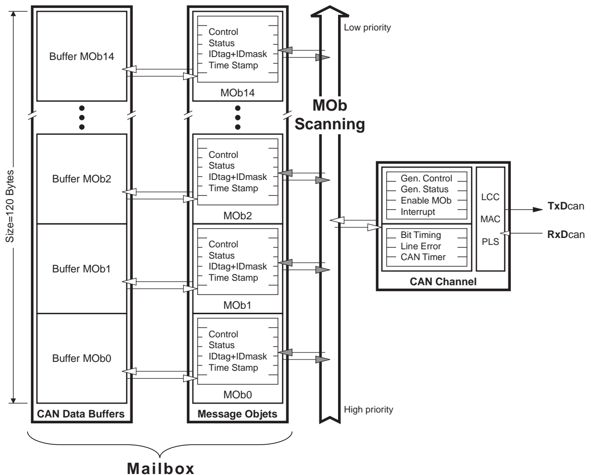
Figure 112. CAN Controller Structure
