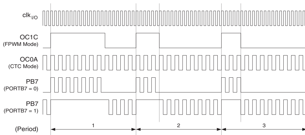
Figure 75. Output Compare Modulator, Timing Diagram
