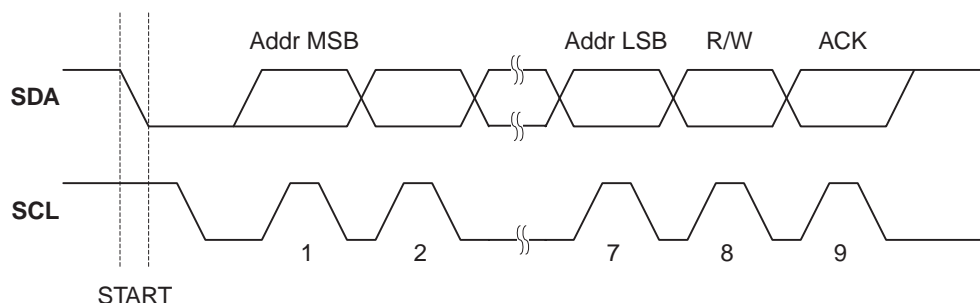
Figure 90. Address Packet Format
