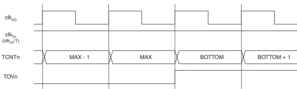
Figure 68. Timer/Counter Timing Diagram, no Prescaling
