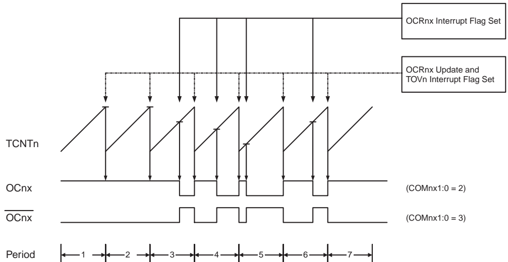
Figure 66. Fast PWM Mode, Timing Diagram
