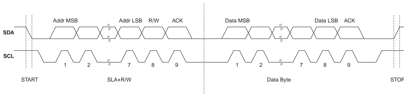
Figure 92. Typical Data Transmission
