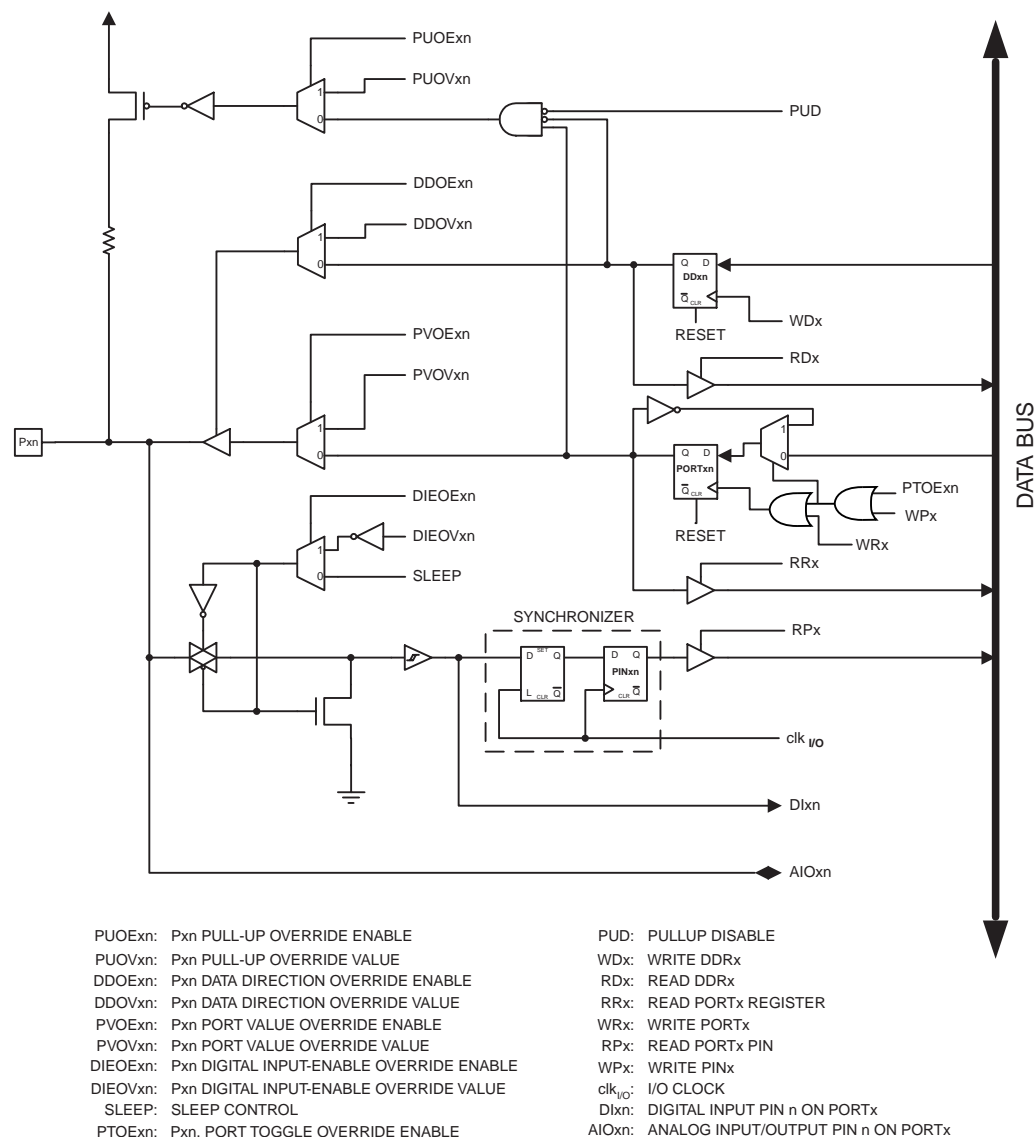
Figure 33. Alternate Port Functions (1)
