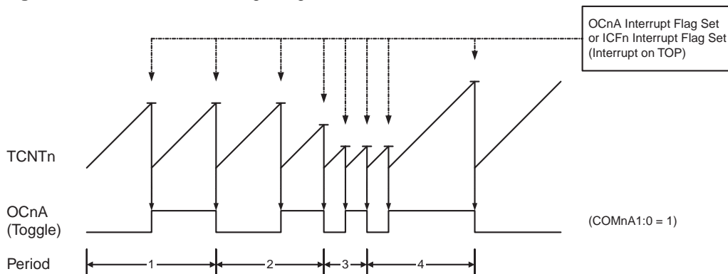
Figure 52. CTC Mode, Timing Diagram
