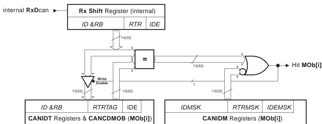
Figure 117. Acceptance Filter Block Diagram
