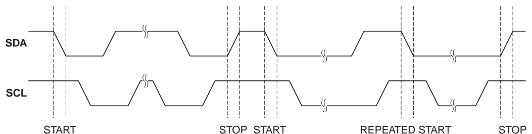
Figure 89. START, REPEATED START and STOP Conditions
