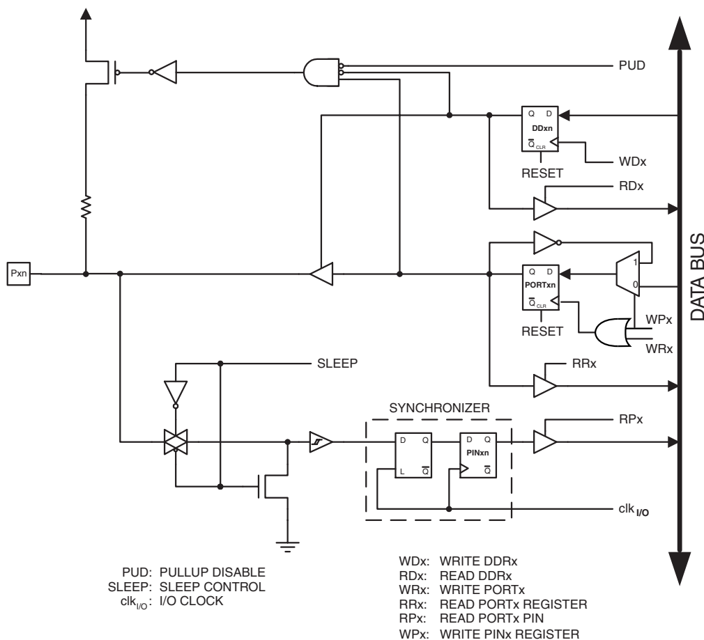
Figure 30. General Digital I/O (1)
