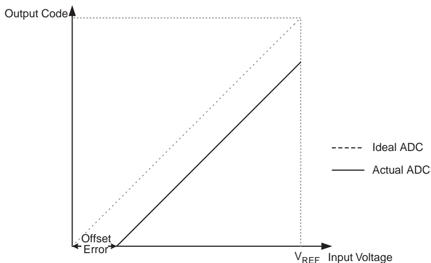
Figure 133. Offset Error
