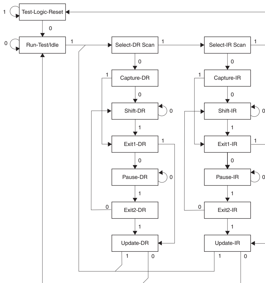
Figure 139. TAP Controller State Diagram
