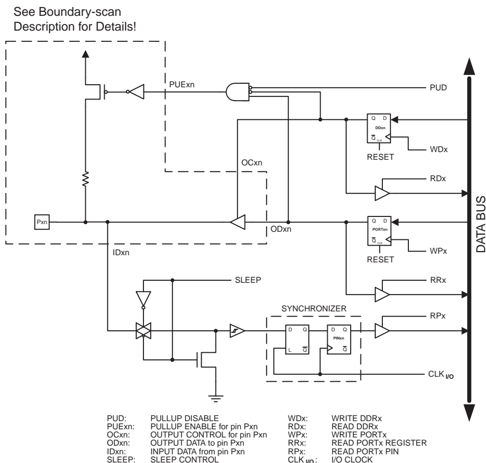
Figure 143. General Port Pin Schematic Diagram
