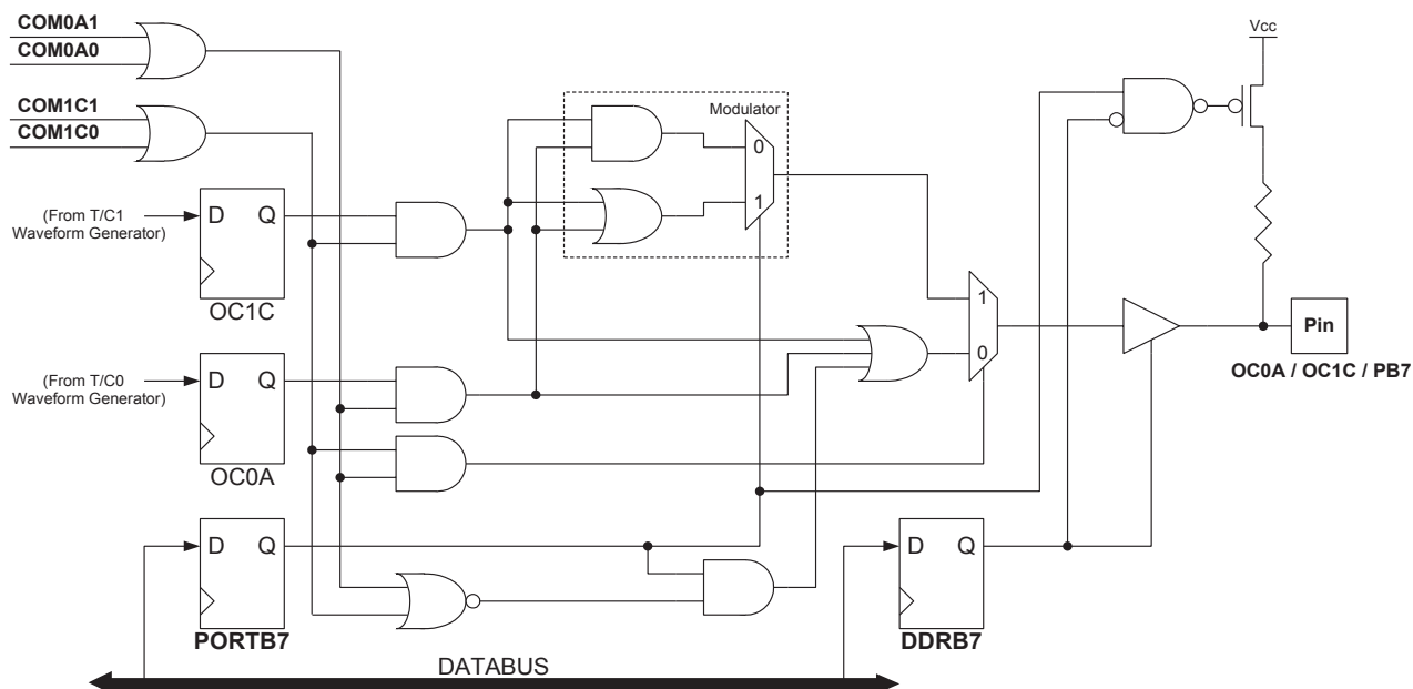
Figure 74. Output Compare Modulator, Schematic
