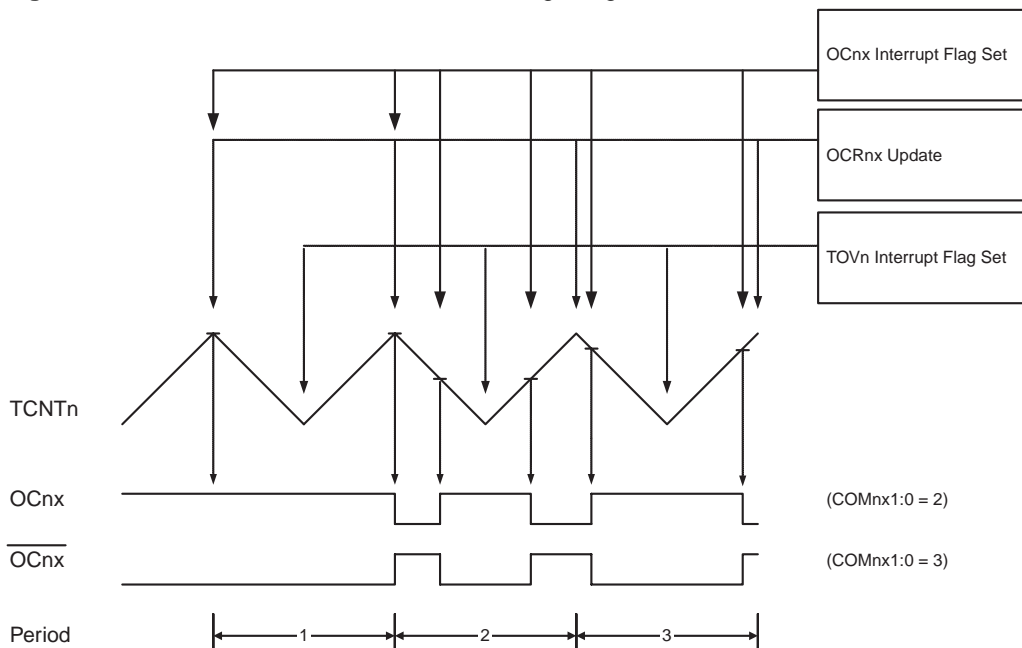
Figure 42. Phase Correct PWM Mode, Timing Diagram
