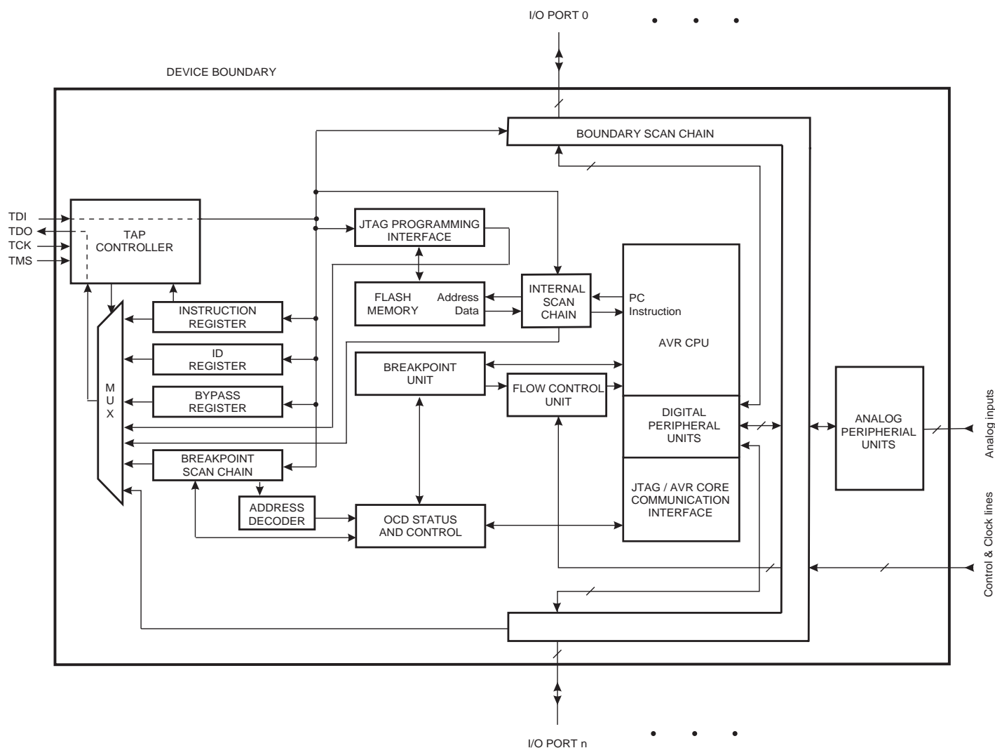
Figure 138. Block Diagram
