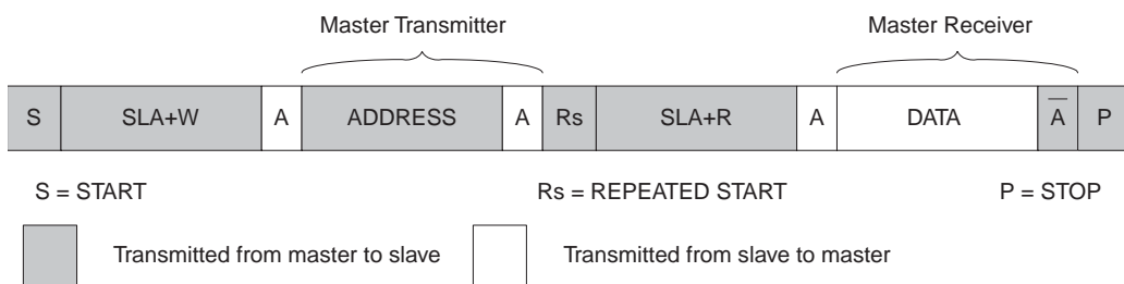
Figure 105. Combining Several TWI Modes to Access a Serial EEPROM
