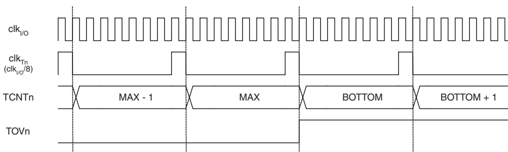
Figure 69. Timer/Counter Timing Diagram, with Prescaler ( f_{\text{clk}_{I/O}/8} )
