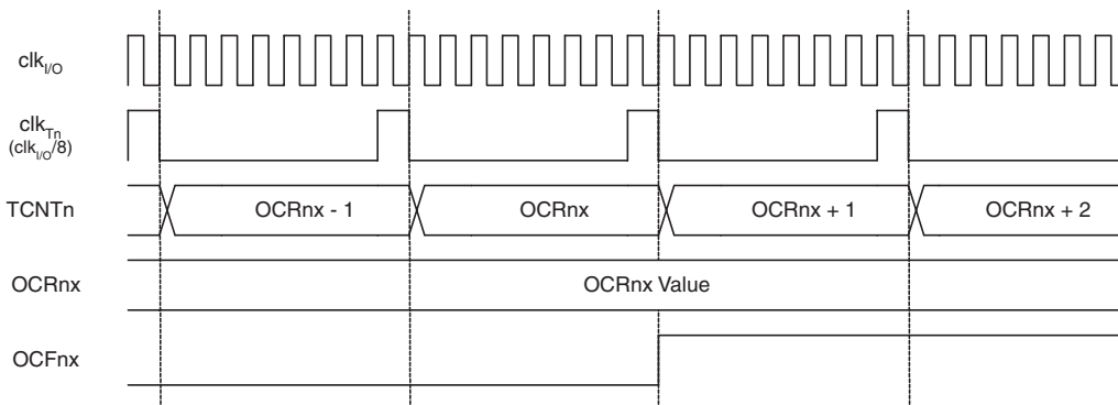
Figure 70. Timer/Counter Timing Diagram, Setting of OCF2A, with Prescaler ( f_{\text{clk}_{I/O}/8} )
