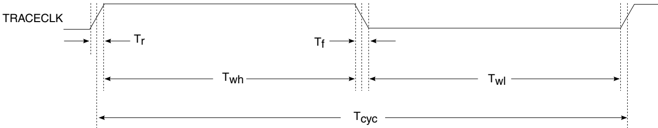
Figure 5. TRACE_CLKOUT specifications
