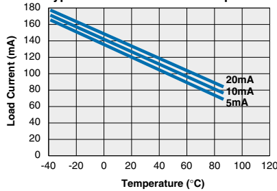
TS120L Typical Load Current vs. Temperature
