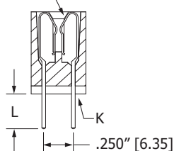
HAIRPIN BELLOWS
