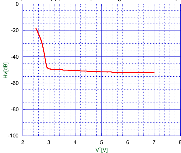
2 nd .Distortion vs. Supply Voltage ( v_{in}=0.5\text{Vpp}, 3.58\text{MHz}, \text{Sine-Signal } \text{RL}=75\text{ohm} )
