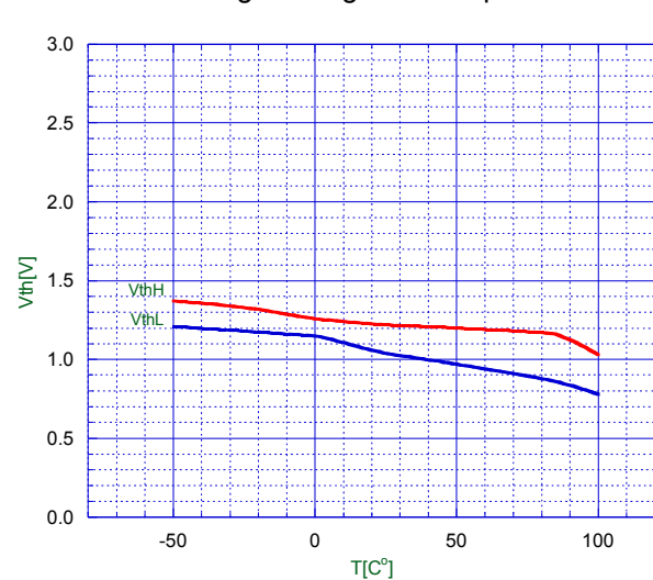
SW Change Voltage vs. Temperature
