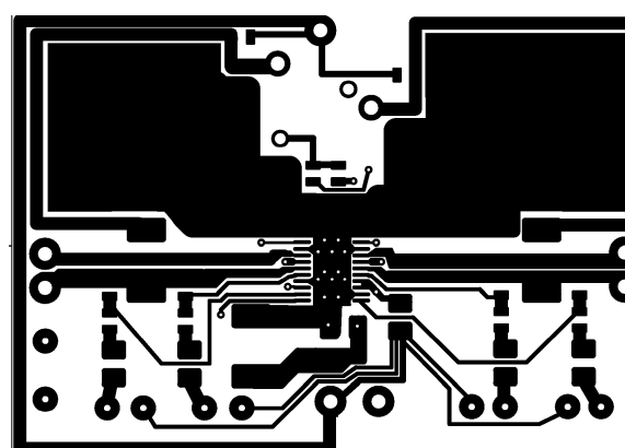
Figure 49. Recommended MTE PC Board Layout: Component-Side Layout
