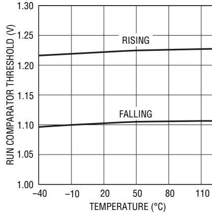
Run Comparator Threshold Voltage vs Temperature
