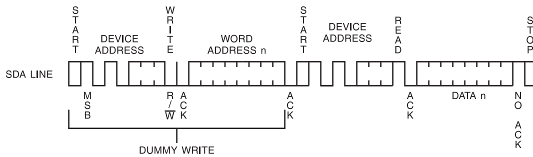
Figure 8-5. Random Read
