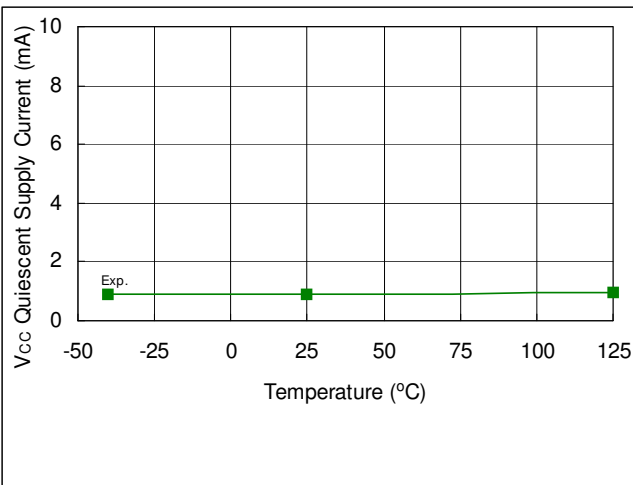
Fig. 36. VCC Quiescent Supply Current vs. Temperature
