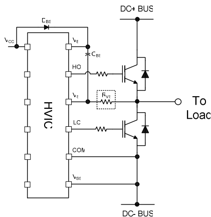
Figure 25: V_S resistor
