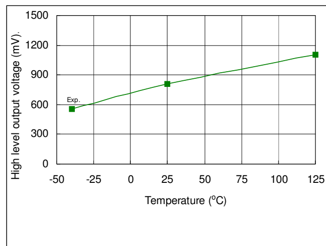
Fig. 42. High Level Output Voltage vs. Temperature
