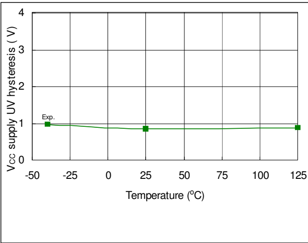
Fig. 34. VCC Supply UV Hysteresis vs. Temperature
