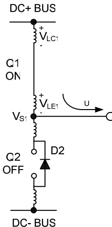
Figure 21: V_S positive
