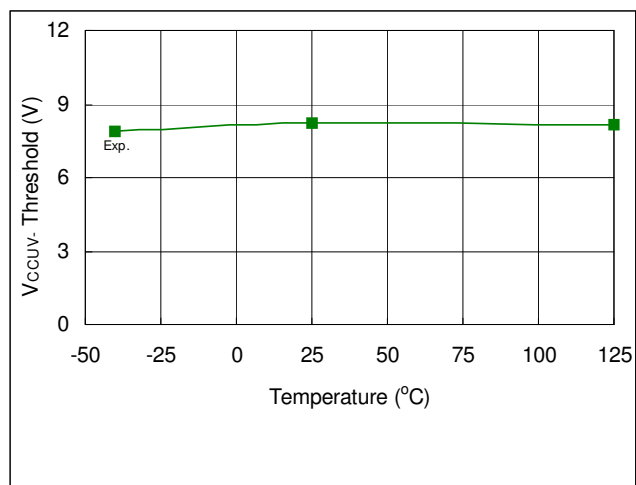
Fig. 39. V_{CCUV-} Threshold vs. Temperature
