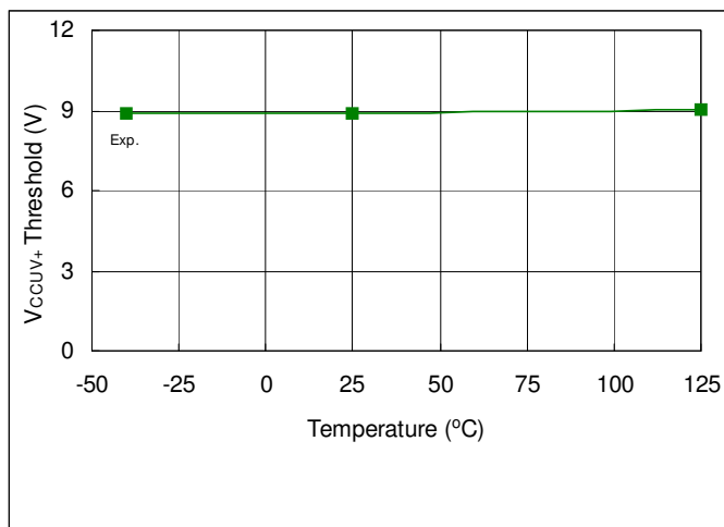
Fig. 38. V_{CCUV+} Threshold vs. Temperature
