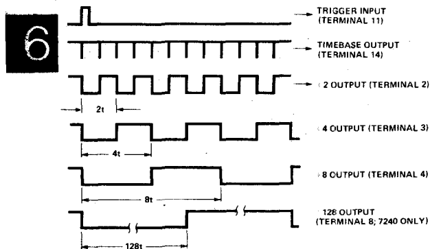
Figure 1. Timing Diagram for ICM7240/50/60
