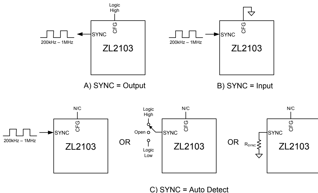
FIGURE 15. SYNC PIN CONFIGURATIONS
