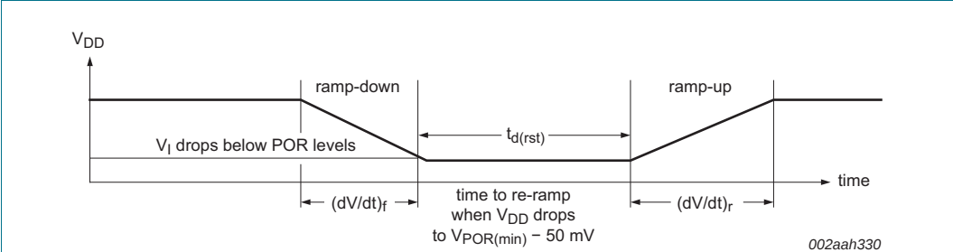
Fig 18. V_{DD} is lowered below the POR threshold, then ramped back up to V_{DD}
