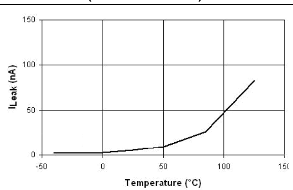
Figure 49. Switch leakage vs. temperature (STMP2161/2171)
