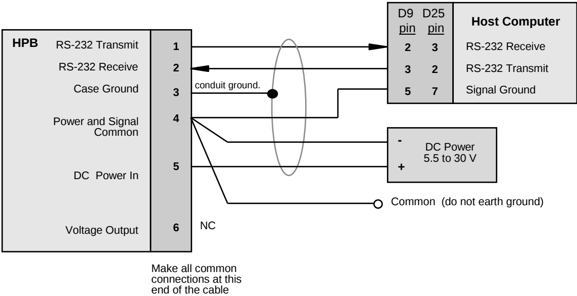
Figure 6.2—Connection for RS-232 Operation
