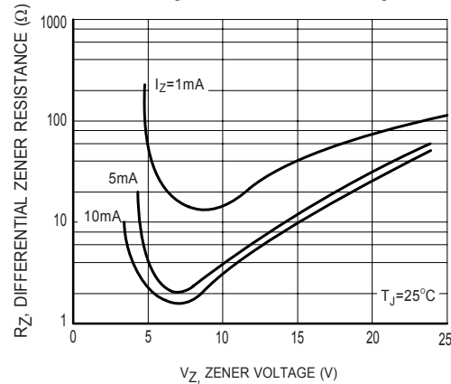
Figure9 Differential Zener Resistance vs. Zener Voltage
