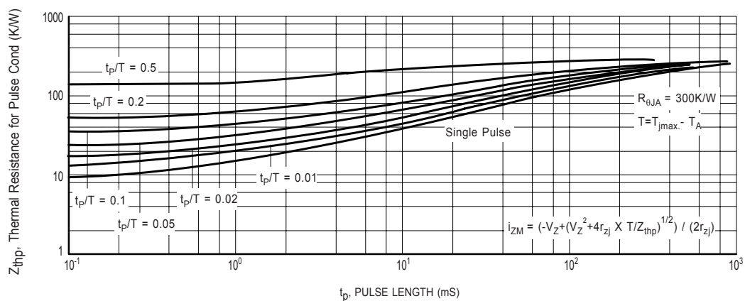
Figure10 Thermal Response
