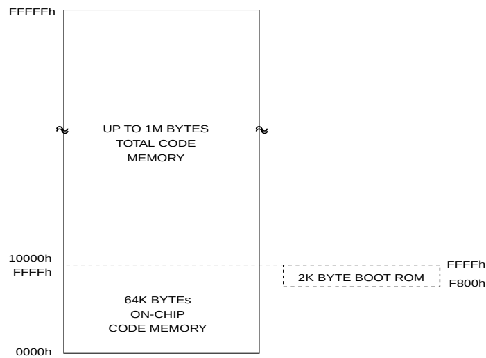
Figure 1. XA Program Memory Map
