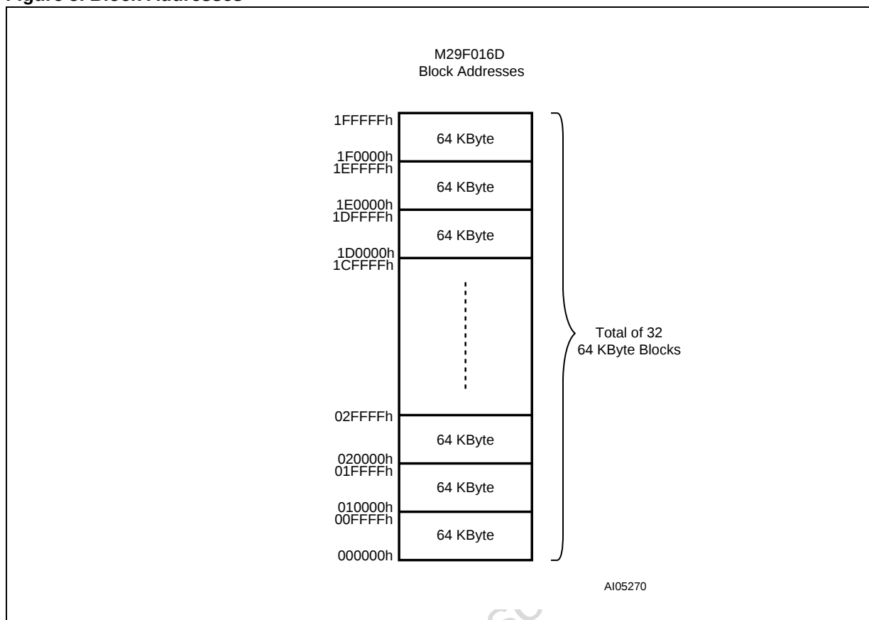
Figure 5. Block Addresses
