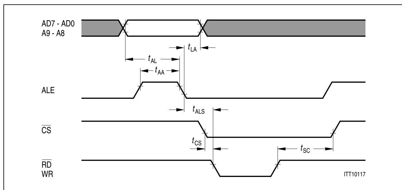
Figure 7-3 Address Timing
