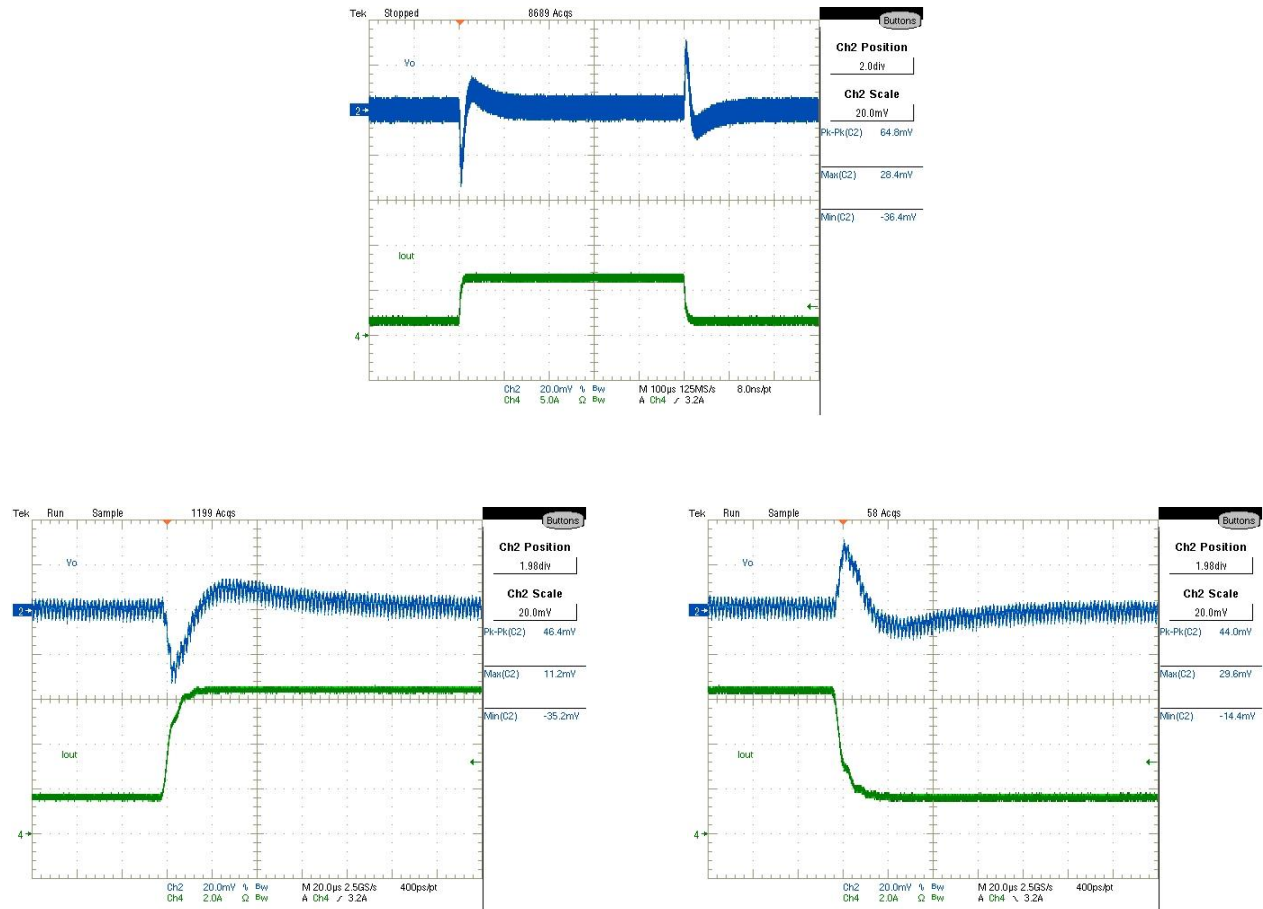
Figure 37: V_{out} Transient Response, 1.6A to 6.4A step at 2.5A/μSec CH2: V_{out} , CH4: I_{out}
