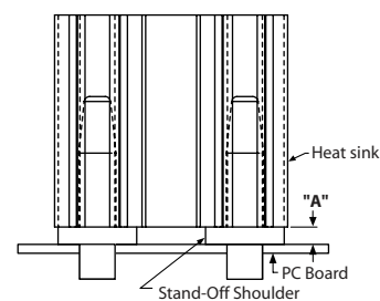
Typical installation P2-P3
