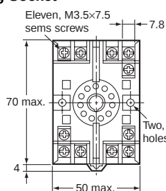
P2CF-11 Front Connecting Socket
