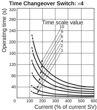
Overcurrent Operating Time Characteristics (Instantaneous Type - Start-up Lock)
