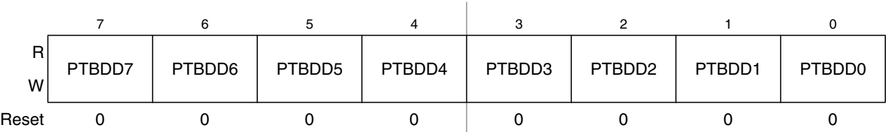
Figure 6-11. Data Direction for Port B (PTBDD)
