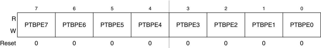
Figure 6-10. Pullup Enable for Port B (PTBPE)
