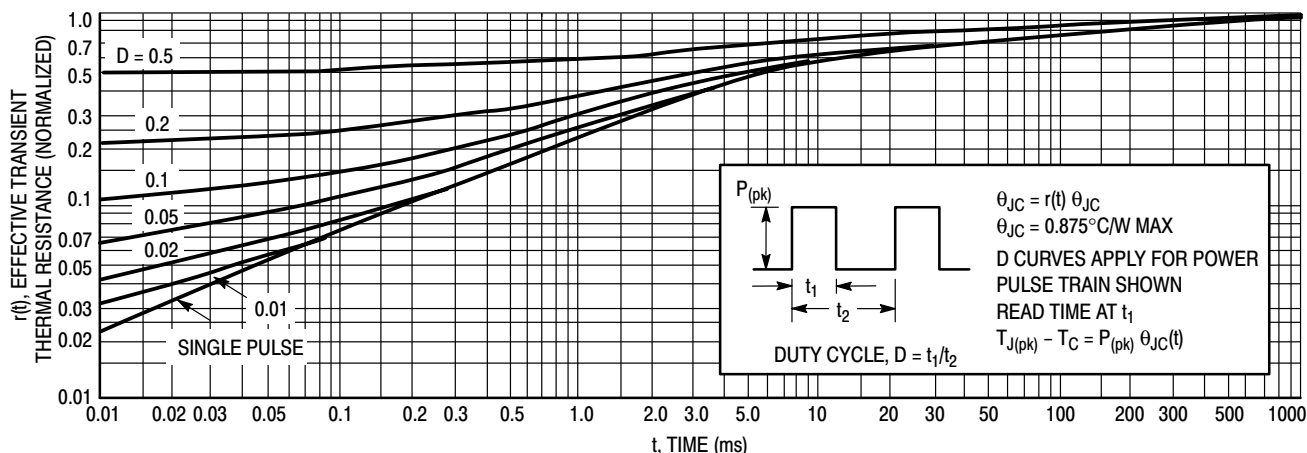
Figure 4. Thermal Response
