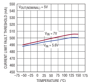
Precision Current Limit, R_{\text{IMAX}} = 604\Omega
