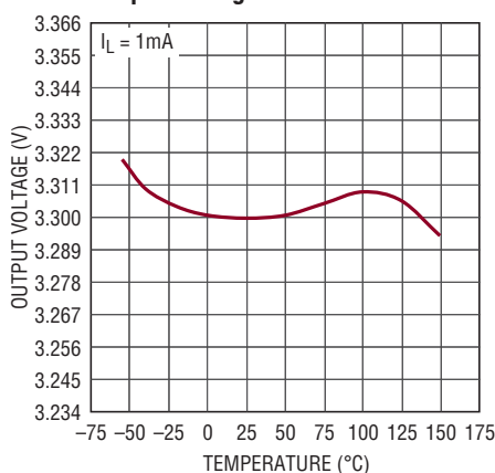
Output Voltage-LT3055-3.3
