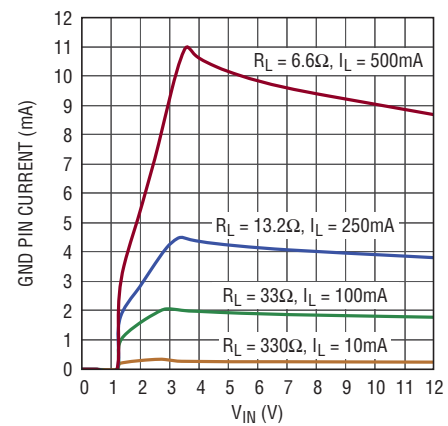
GND Pin Current-LT3055-3.3
