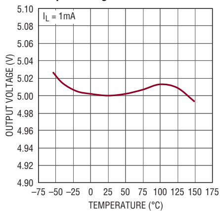
Output Voltage-LT3055-5
