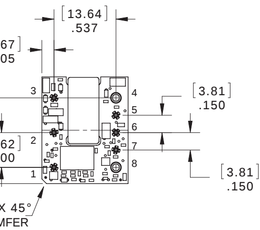
BOTTOM PIN SIDE VIEW
