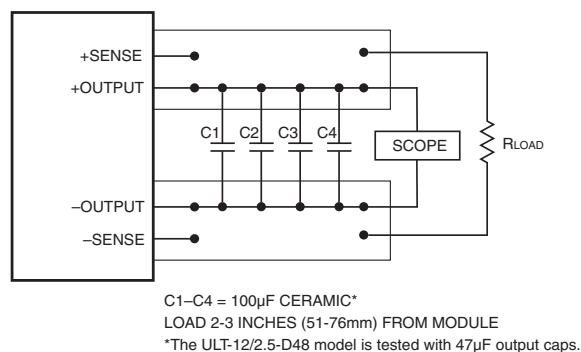
Figure 3. Measuring Output Ripple/Noise (PARD)
