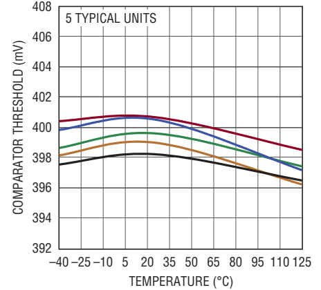
Comparator Threshold vs Temperature
