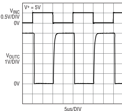
LT6108-2 Comparator Step Response (100mV INC Overdrive)
