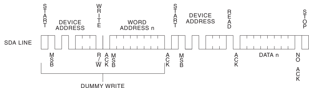
Figure 8-2. Random Read
