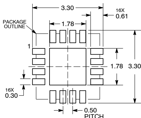
RECOMMENDED SOLDERING FOOTPRINT*
