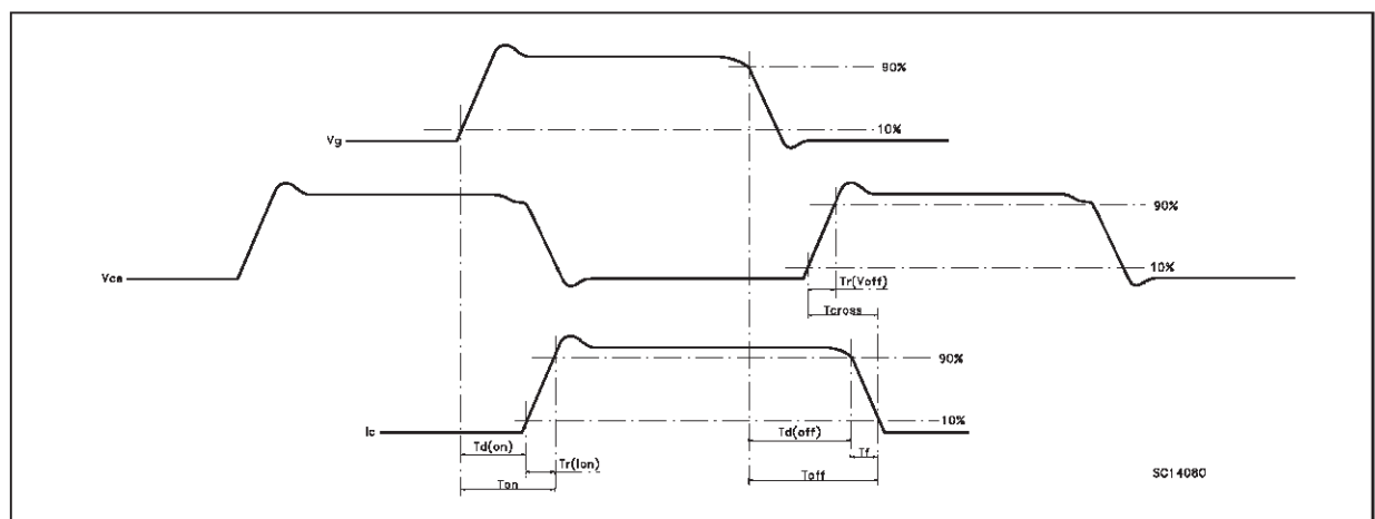
Fig. 3: Switching Waveforms
