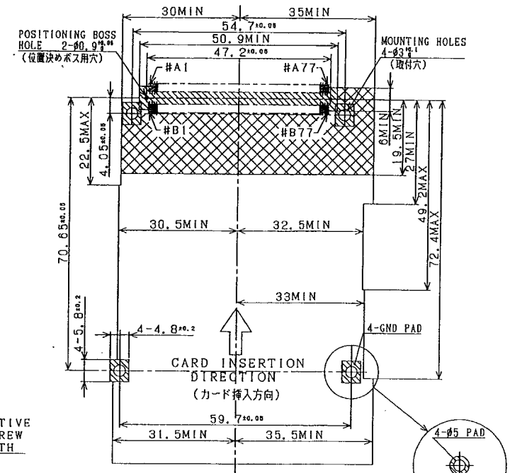
RECOMMENDED P.C. BOARD LAYOUT (MOUNTING FACE SIDE)
