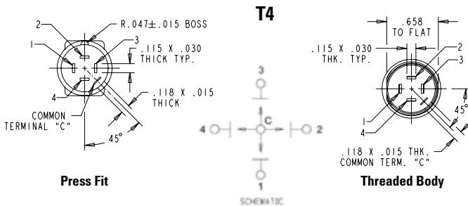
Threaded Body
