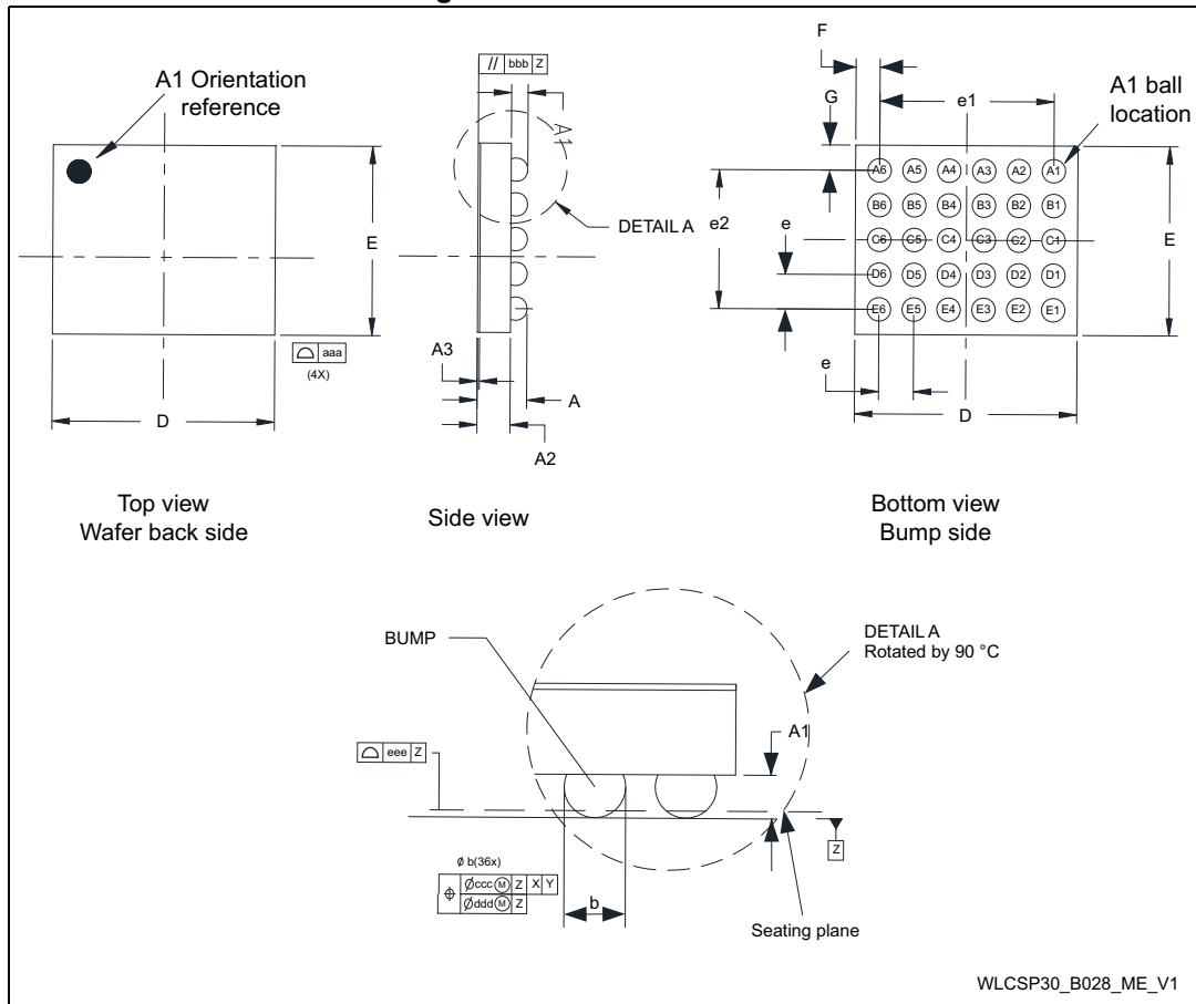
Figure 33. WLCSP30 outline
