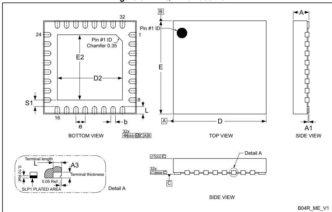
Figure 31. VFQFPN32 outline
