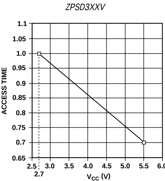
Figure 19. Normalized Access Time ( T_6 ) ( V_{CC} = 3.0\text{ V} )
