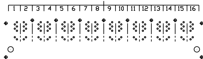
PORT ASSIGNMENT (COMPONENT SIDE VIEW)
