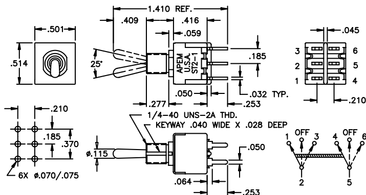
DOUBLE POLE
