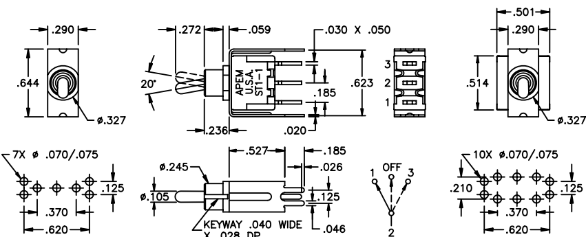
SINGLE POLE
