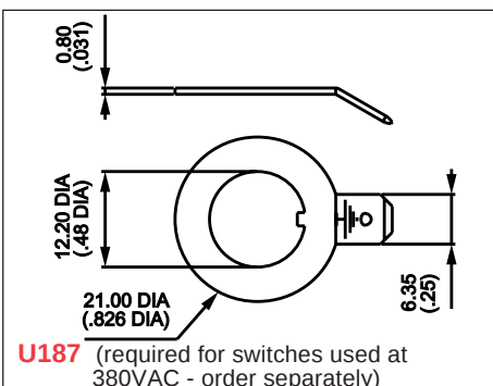
600H/2 Solder lug terminals
