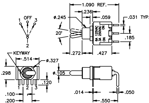
SINGLE POLE
