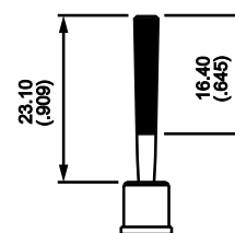
21 Specify U640 insulative extension with this actuator and replace '0' with color selection below.
