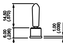
13 for smooth bushing models Cap U1040 is required
