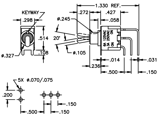
SINGLE POLE
