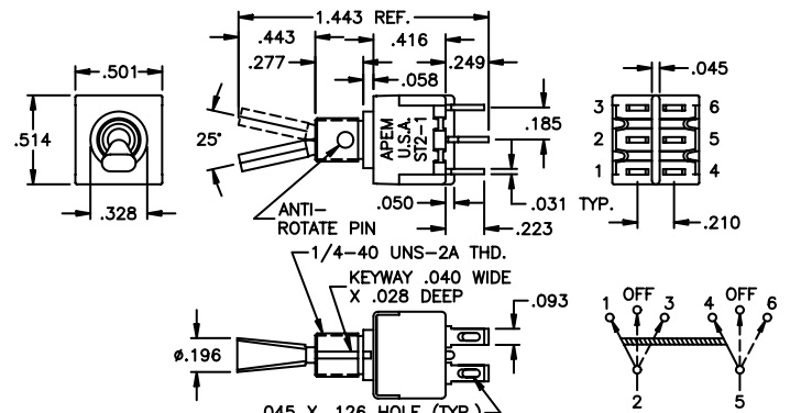
DOUBLE POLE
