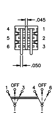
DOUBLE POLE
