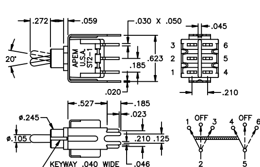
DOUBLE POLE
