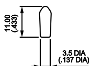
U270 for threaded bushing models
