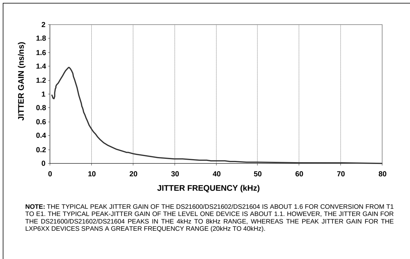
Figure 3-1. Nominal Jitter Transfer for 2.048MHz-to-1.544MHz Conversion
