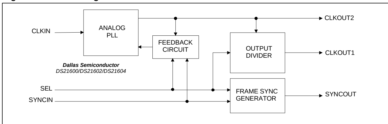
Figure 1-1. Block Diagram
