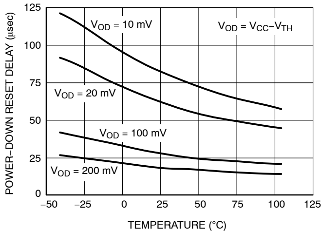
Figure 12. Power-Down Reset Delay vs. Temperature and Overdrive ( V_{TH} = 1.2\text{ V} )
