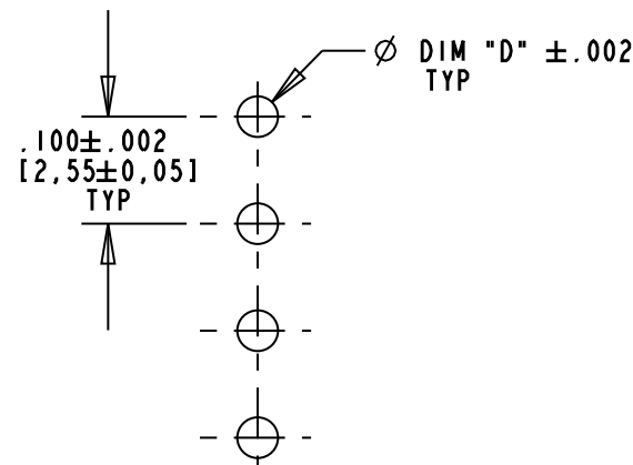
RECOMMENDED HOLE PATTERN GAUGE
