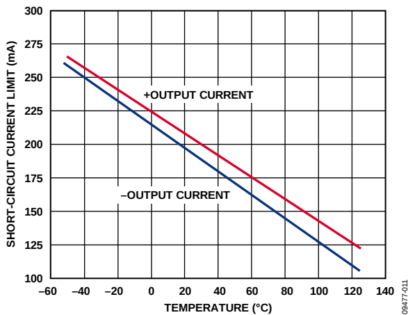
Figure 11. Short-Circuit Current Limit vs. Temperature
