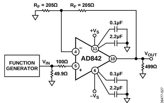
Figure 27. Noninverting Amplifier Configuration (PDIP)
