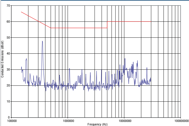
NPH25S4803
