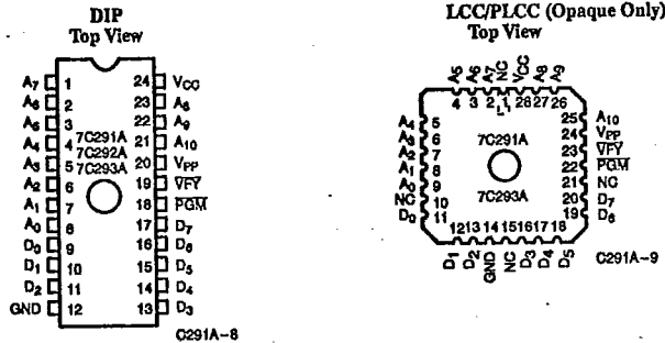
Figure 1. Programming Pinouts
