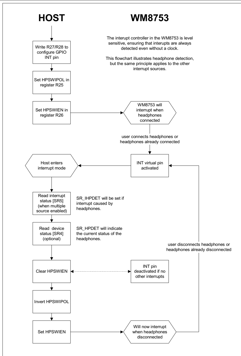
Figure 14 Interrupt Control Flowchart
