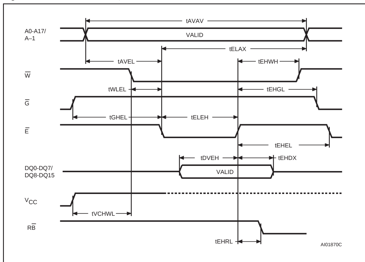
Figure 8. Write AC Waveforms, \overline{E} Controlled
