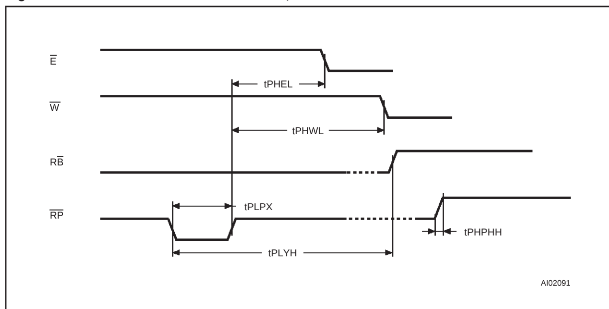
Figure 9. Read and Write AC Characteristics, \overline{R} Related
