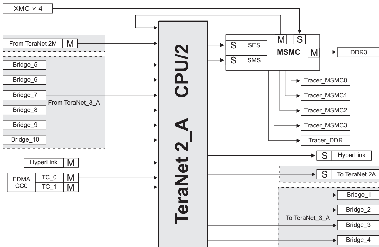
Figure 4-2 TeraNet 2A
