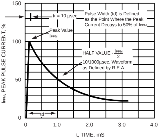
FIG. 3 - PULSE WAVEFORM
