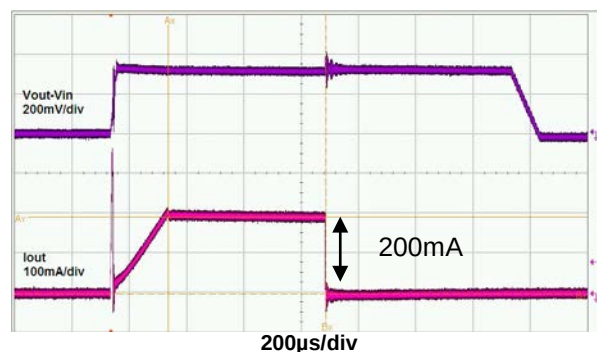
Reverse-Current Limit
